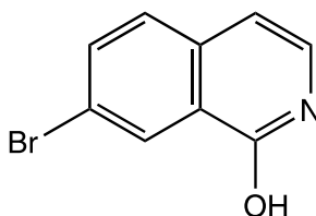
L17800 7-Bromo-1-hydroxyisoquinoline
