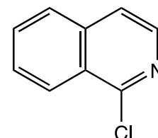
L17831 1-Chloroisoquinoline
