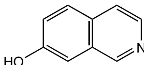
L17067 7-Hydroxyisoquinoline
