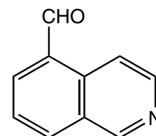
L19636 Isoquinoline-5-carboxaldehyde
