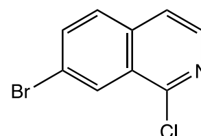
L19946 7-Bromo-1-chloroisoquinoline
