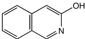
L19428 3-Hydroxyisoquinoline
