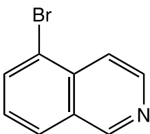
L19632 5-Bromoisoquinoline
