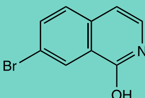
L17800 7-Bromo-1-hydroxyisoquinoline
