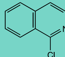
L17831 1-Chloroisoquinoline
