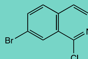
L19946 7-Bromo-1-chloroisoquinoline
