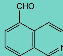
L19636 Isoquinoline-5-carboxaldehyde
