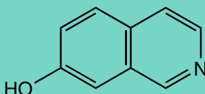
L17067 7-Hydroxyisoquinoline
